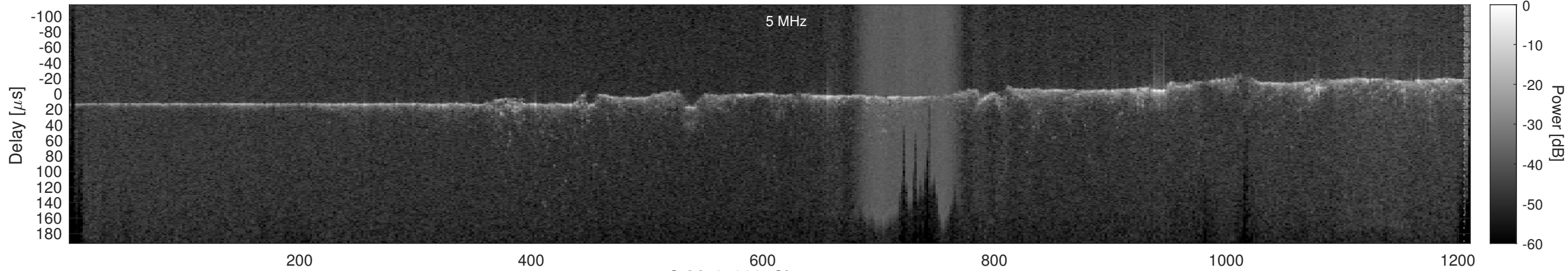
Orbit 21992, Cluttergram
