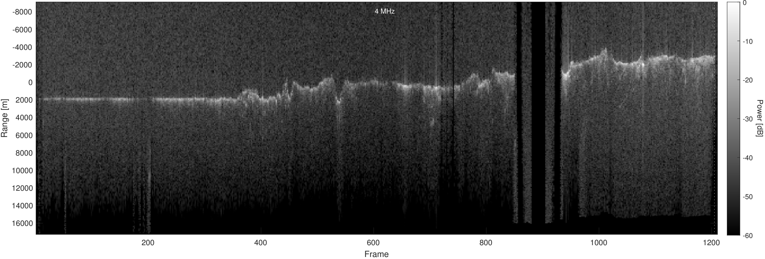
Orbit 21992, Optimized, No Window, Depth-Corrected, Channel 2
