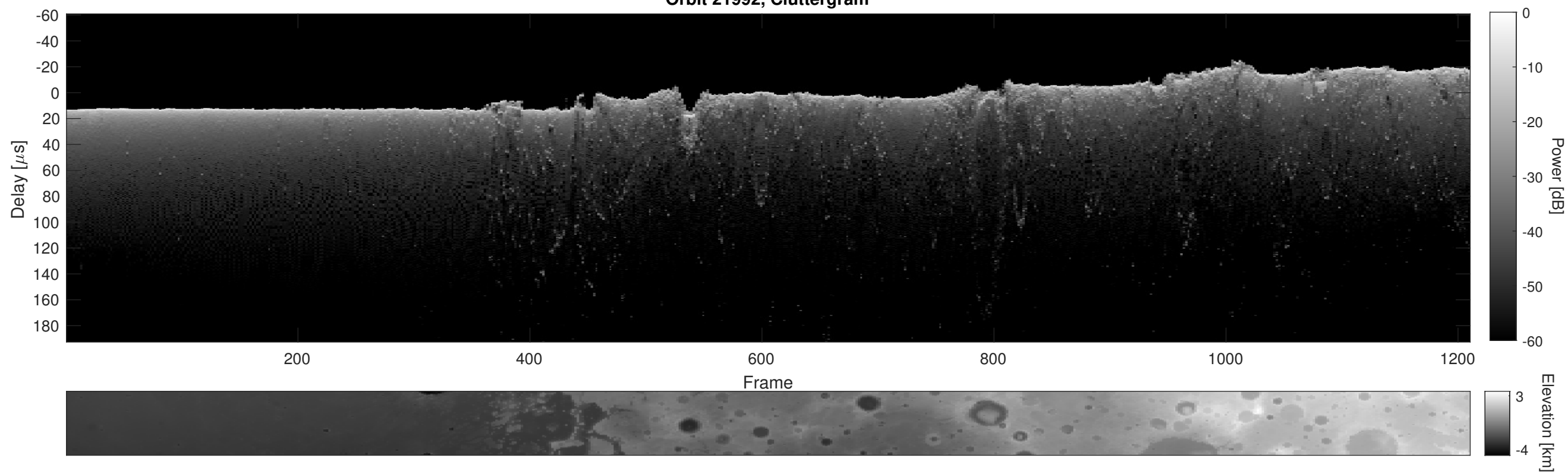
Orbit 21992, Cluttergram
