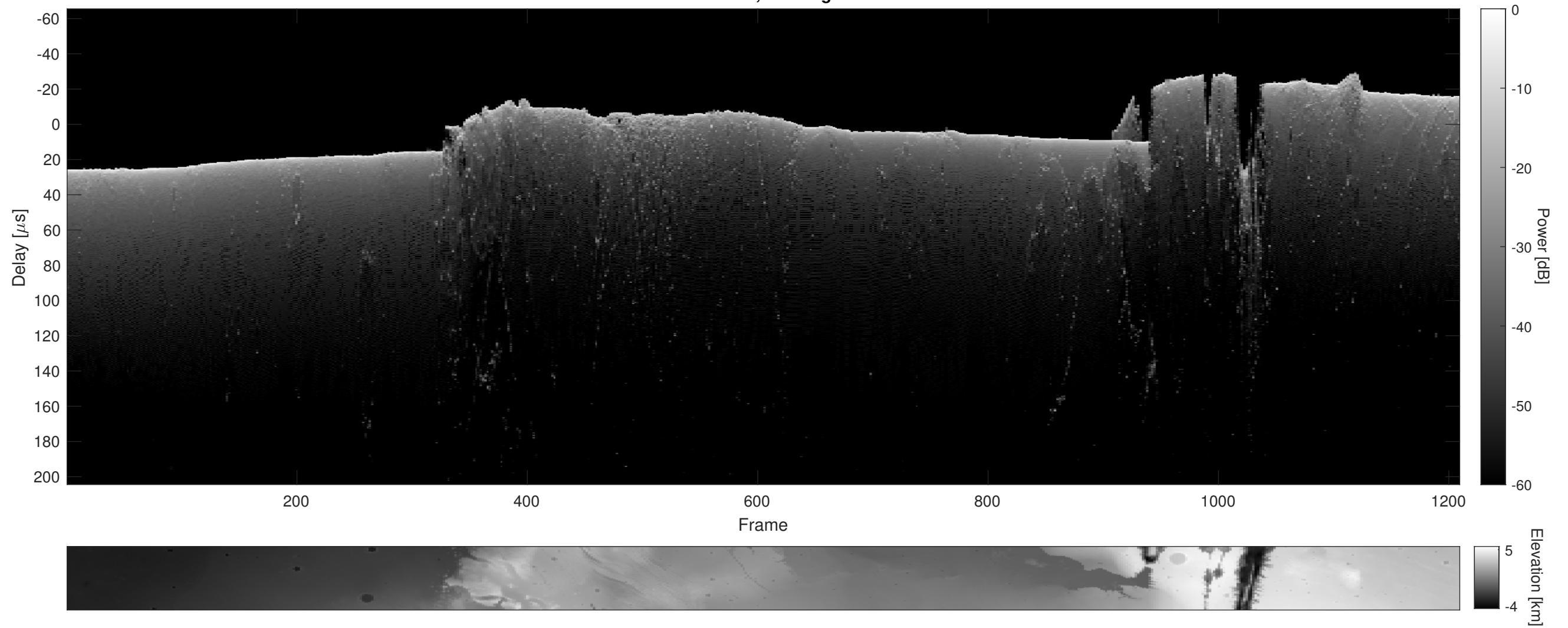
Orbit 21993, Cluttergram
