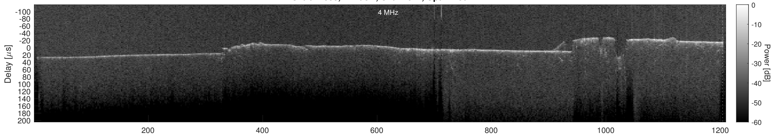
Orbit 21993, Cluttergram
