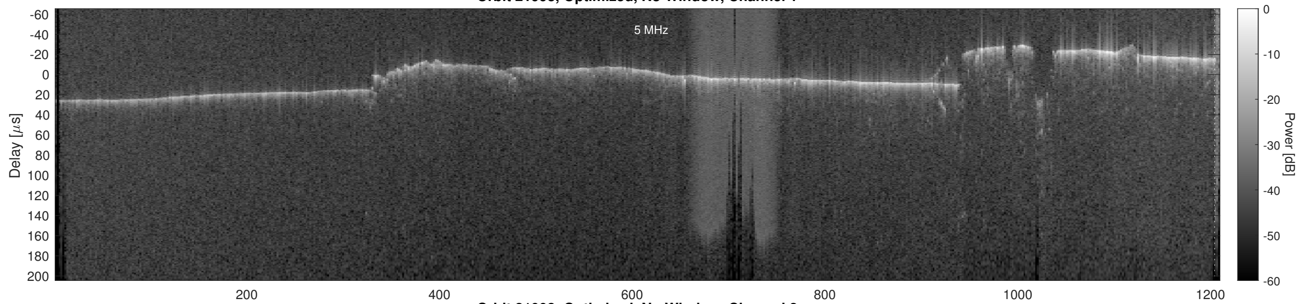
Orbit 21993, Optimized, No Window, Channel 2
