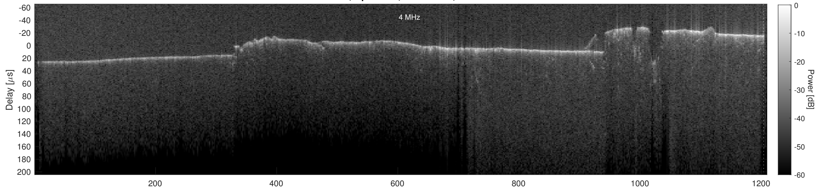
Orbit 21993, Cluttergram
