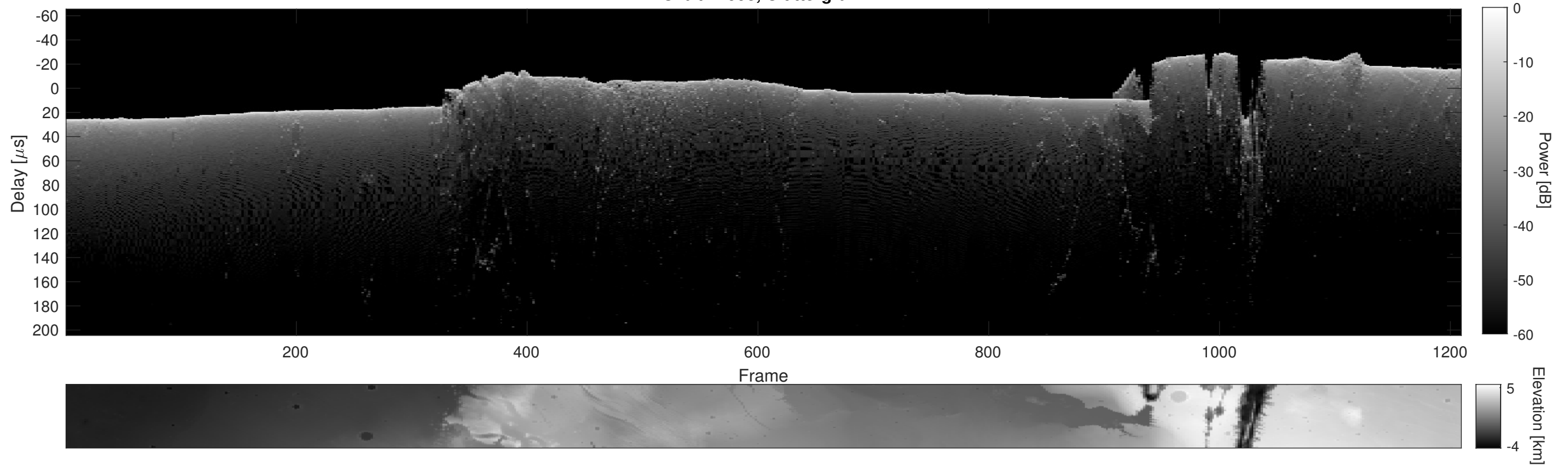
Orbit 21993, Cluttergram
