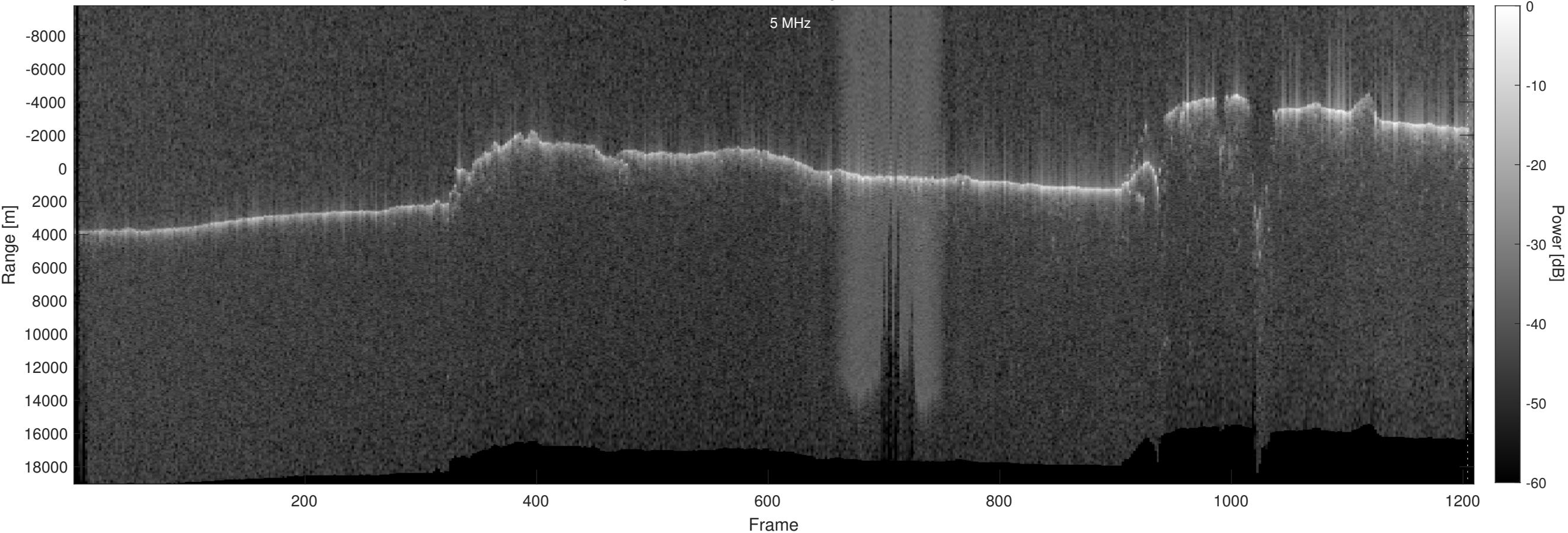
Orbit 21993, Optimized, No Window, Depth-Corrected, Channel 2
