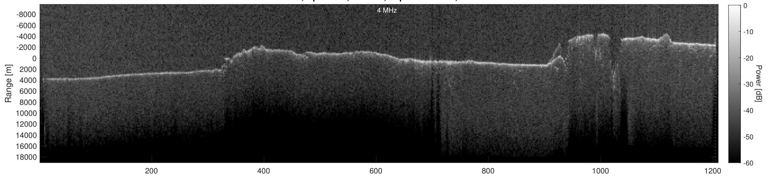
Orbit 21993, Depth-Corrected Cluttergram
