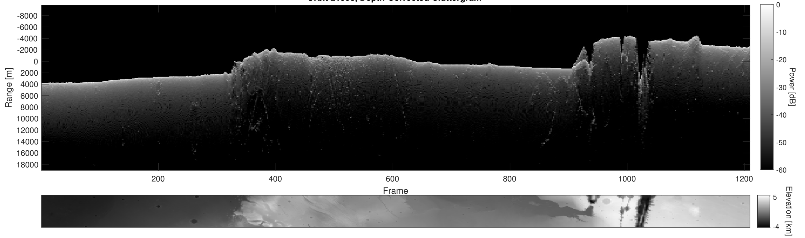
Orbit 21993, Depth-Corrected Cluttergram
