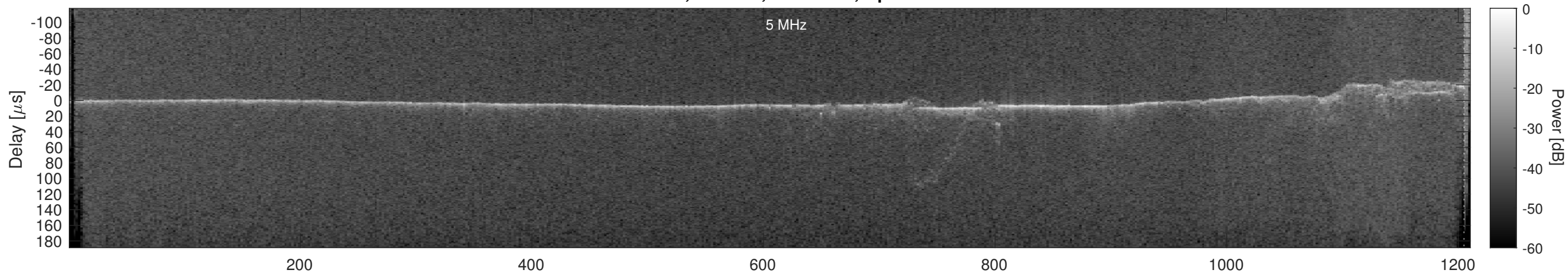
Orbit 21994, Cluttergram
