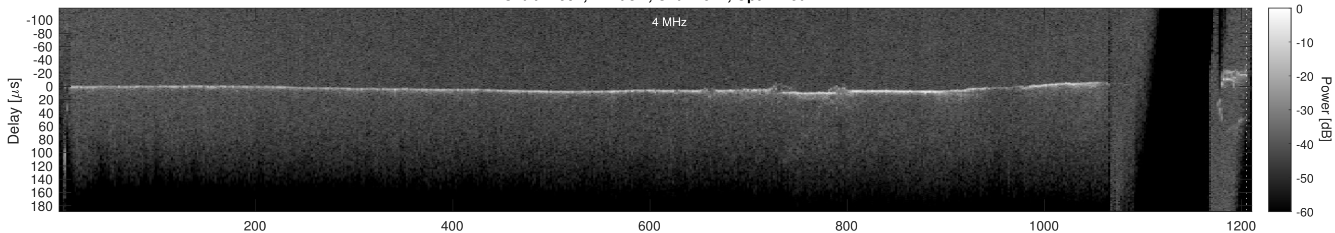
Orbit 21994, Cluttergram
