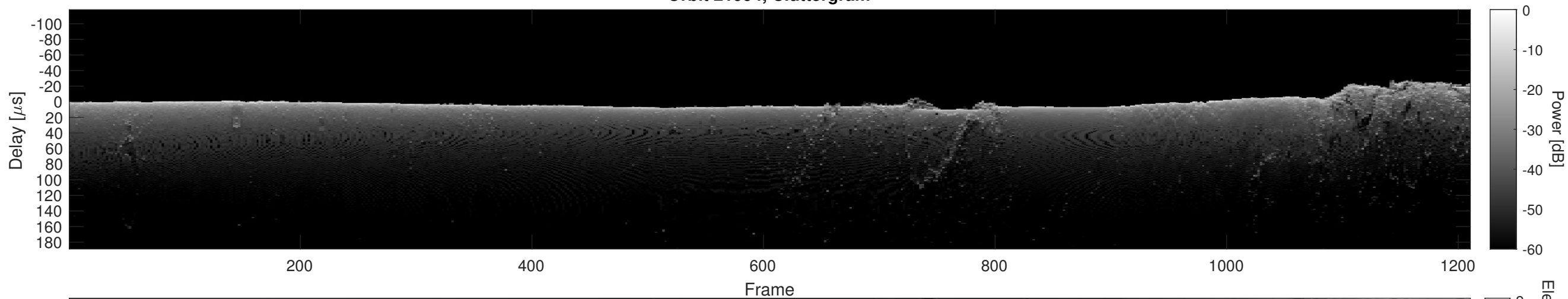
Orbit 21994, Cluttergram
