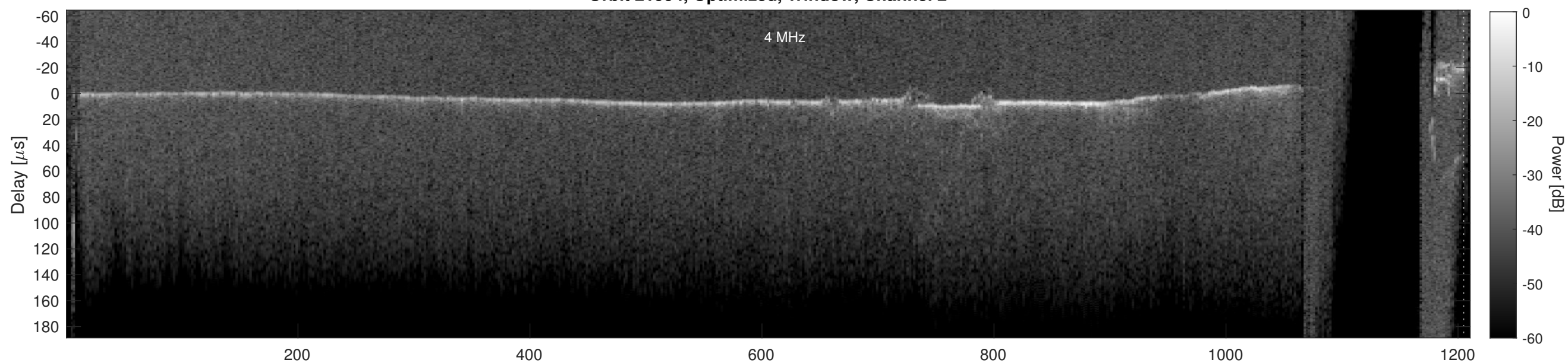
Orbit 21994, Cluttergram
