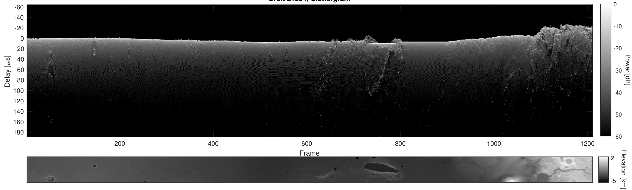
Orbit 21994, Cluttergram
