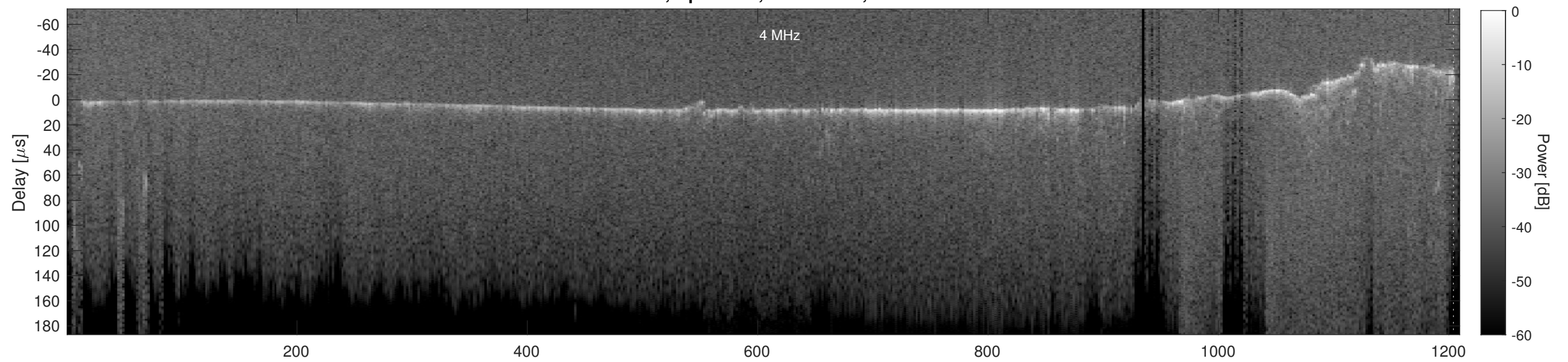
Orbit 22001, Cluttergram
