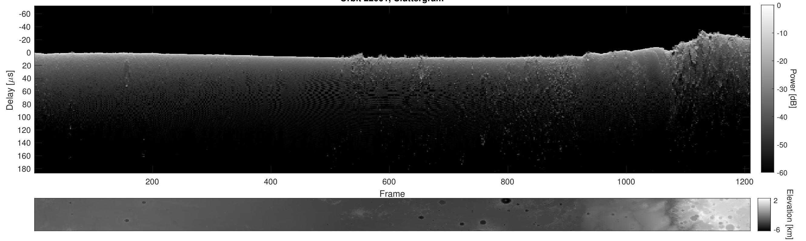
Orbit 22001, Cluttergram
