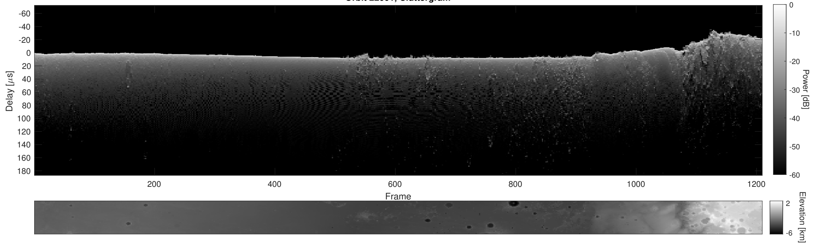
Orbit 22001, Cluttergram
