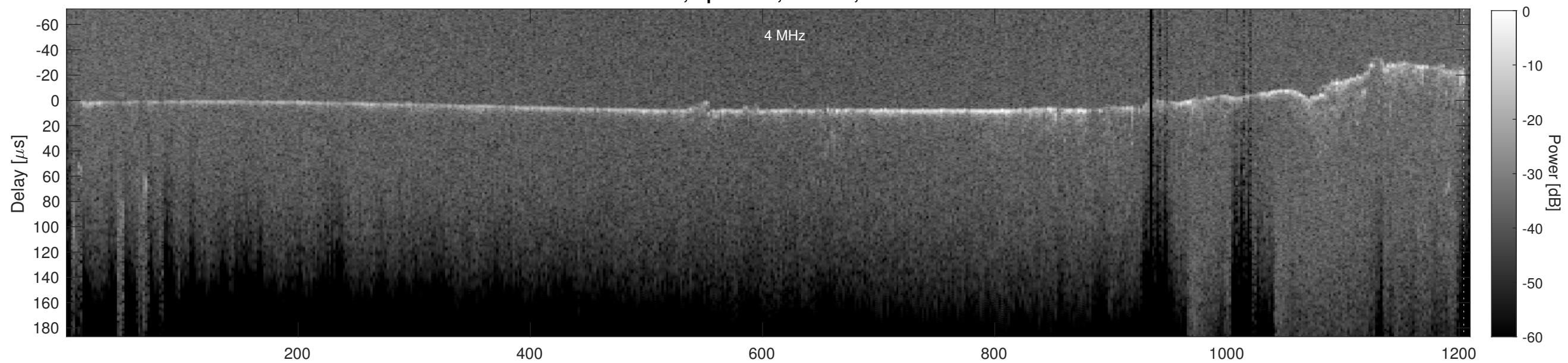
Orbit 22001, Cluttergram
