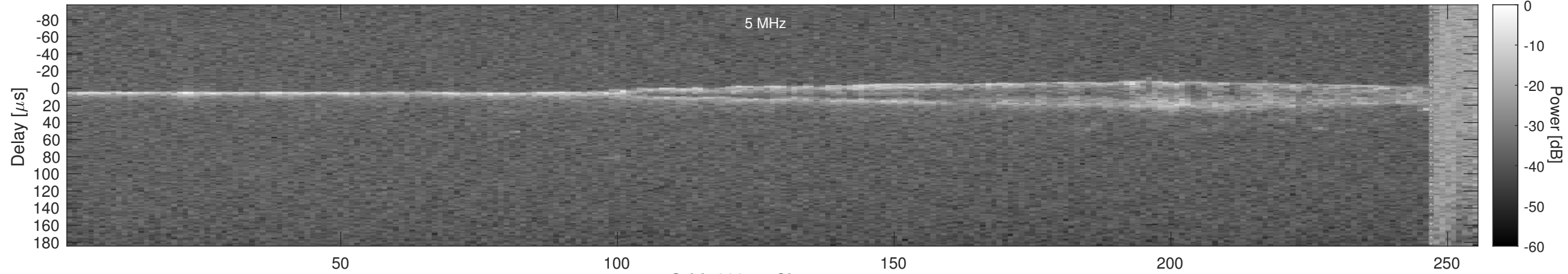
Orbit 22251, Cluttergram
