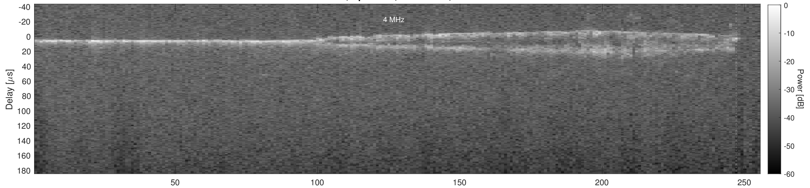
Orbit 22251, Cluttergram
