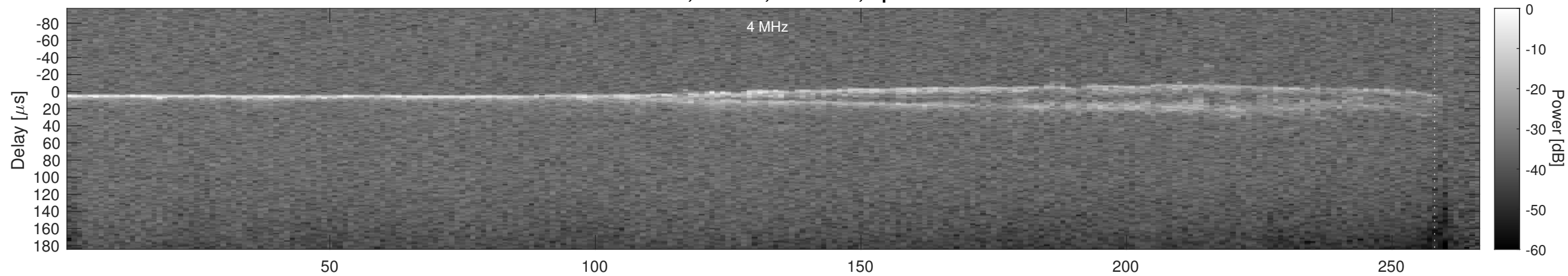
Orbit 22258, Cluttergram
