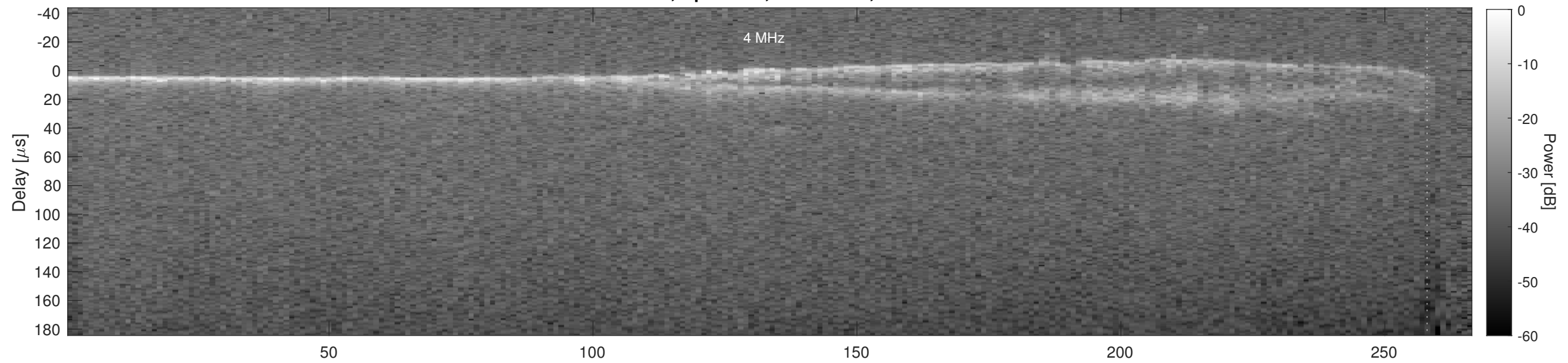
Orbit 22258, Cluttergram
