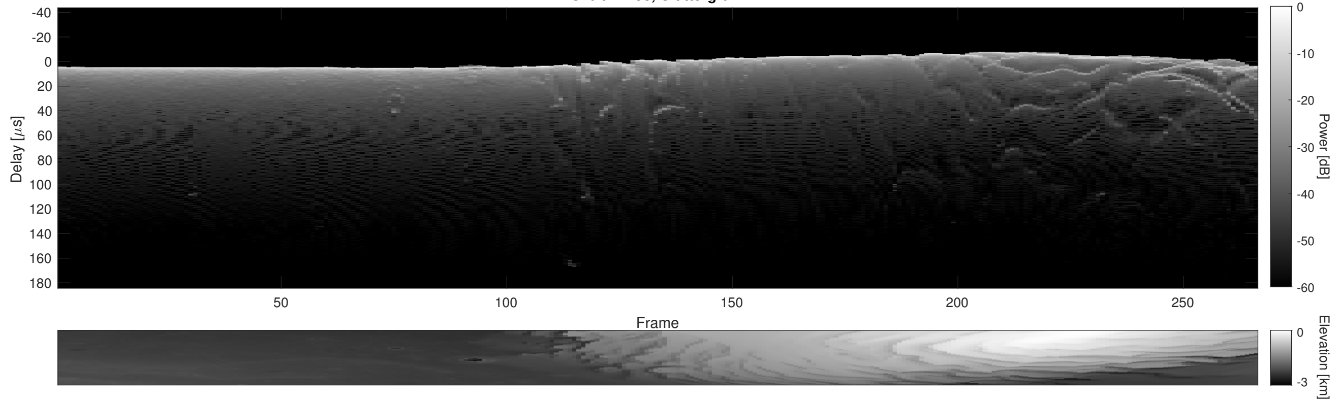
Orbit 22258, Cluttergram
