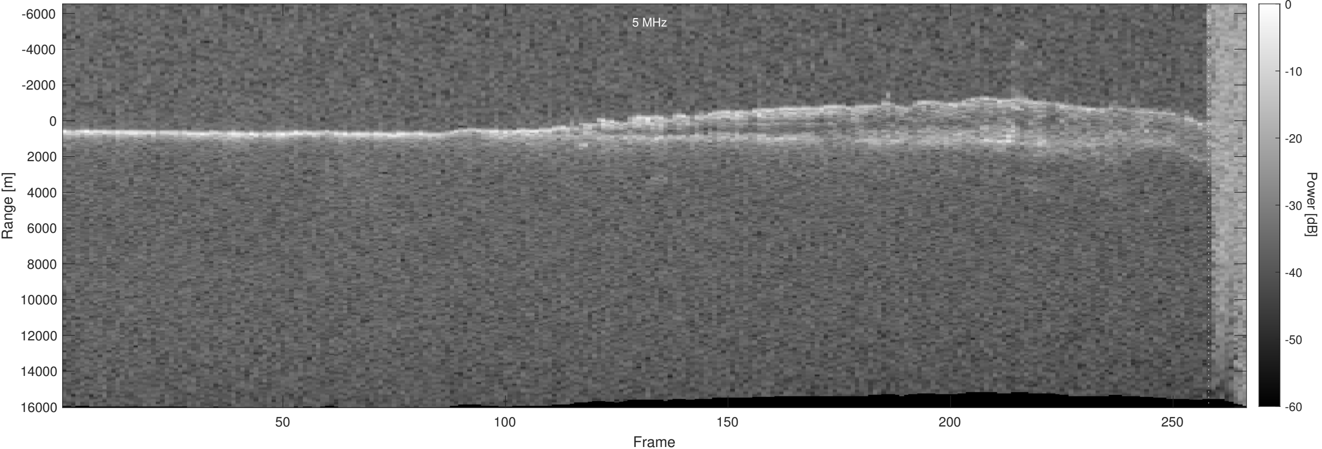
Orbit 22258, Optimized, Window, Depth-Corrected, Channel 2
