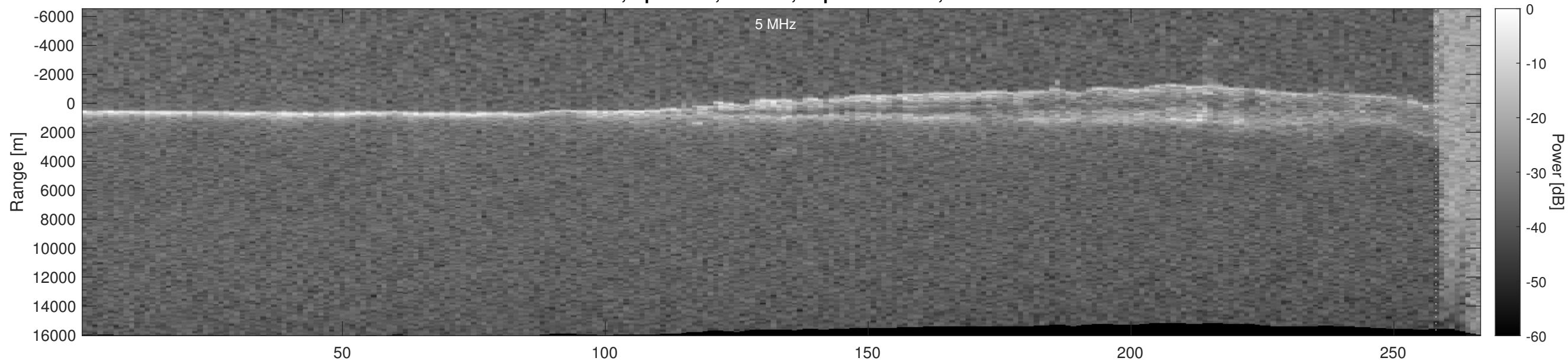
Orbit 22258, Optimized, Window, Depth-Corrected, Channel 2
