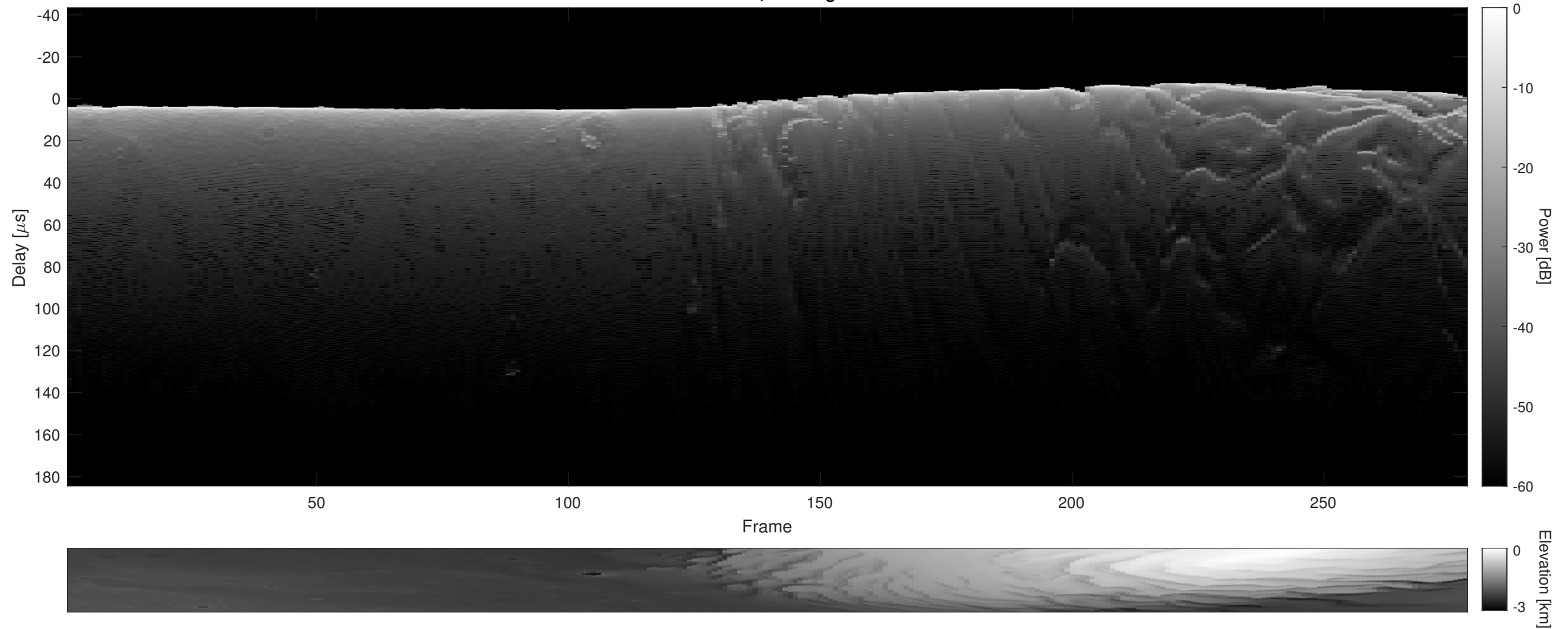
Orbit 22265, Cluttergram
