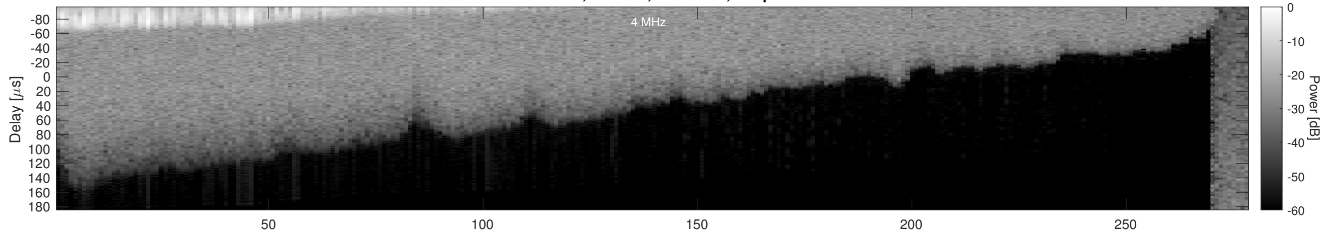
Orbit 22265, Window, Channel 2, Optimized
