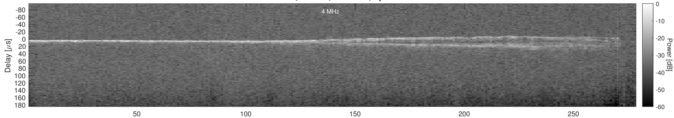
Orbit 22265, Cluttergram
