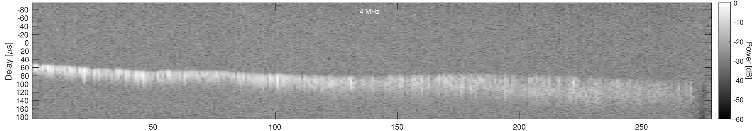
Orbit 22265, Window, Channel 2, Chapman
