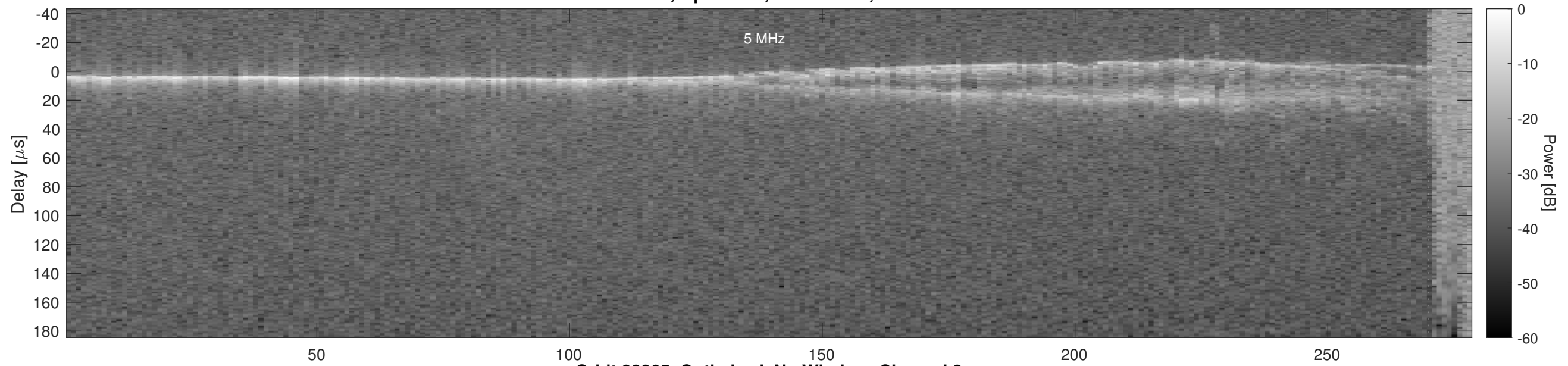
Orbit 22265, Optimized, No Window, Channel 2
