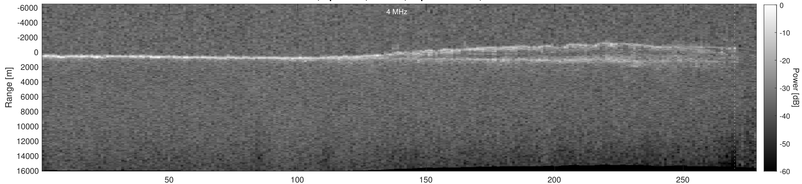
Orbit 22265, Depth-Corrected Cluttergram
