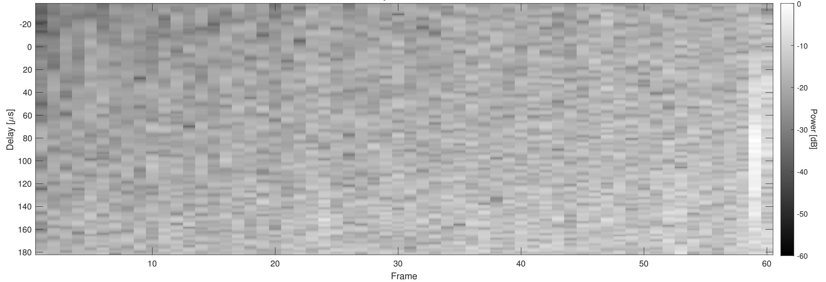
Orbit 22271, Chapman, Window, Channel 2
