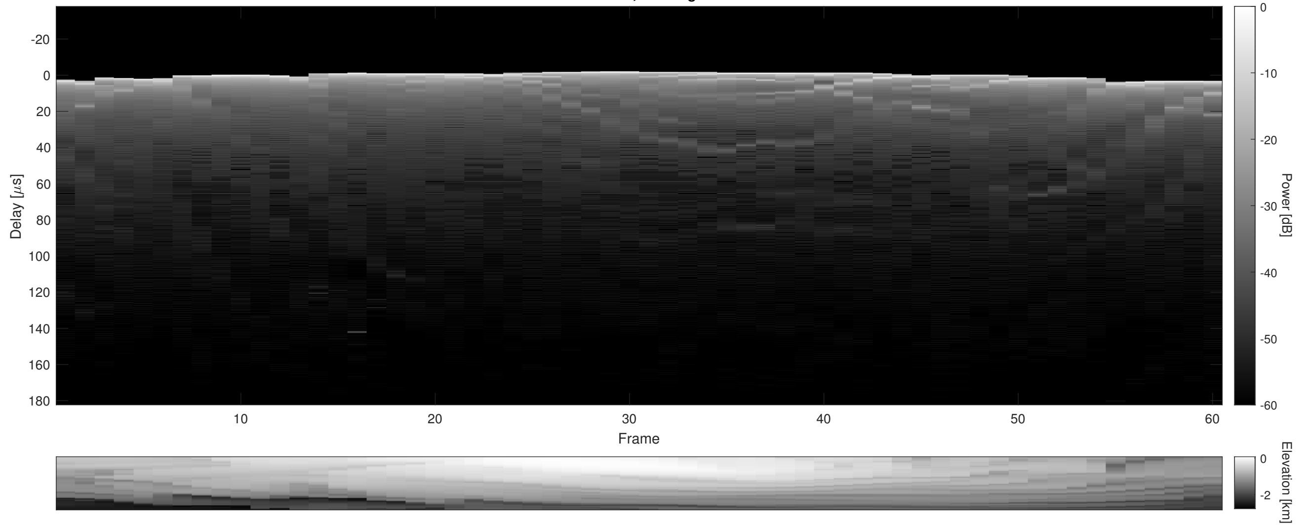
Orbit 22271, Cluttergram
