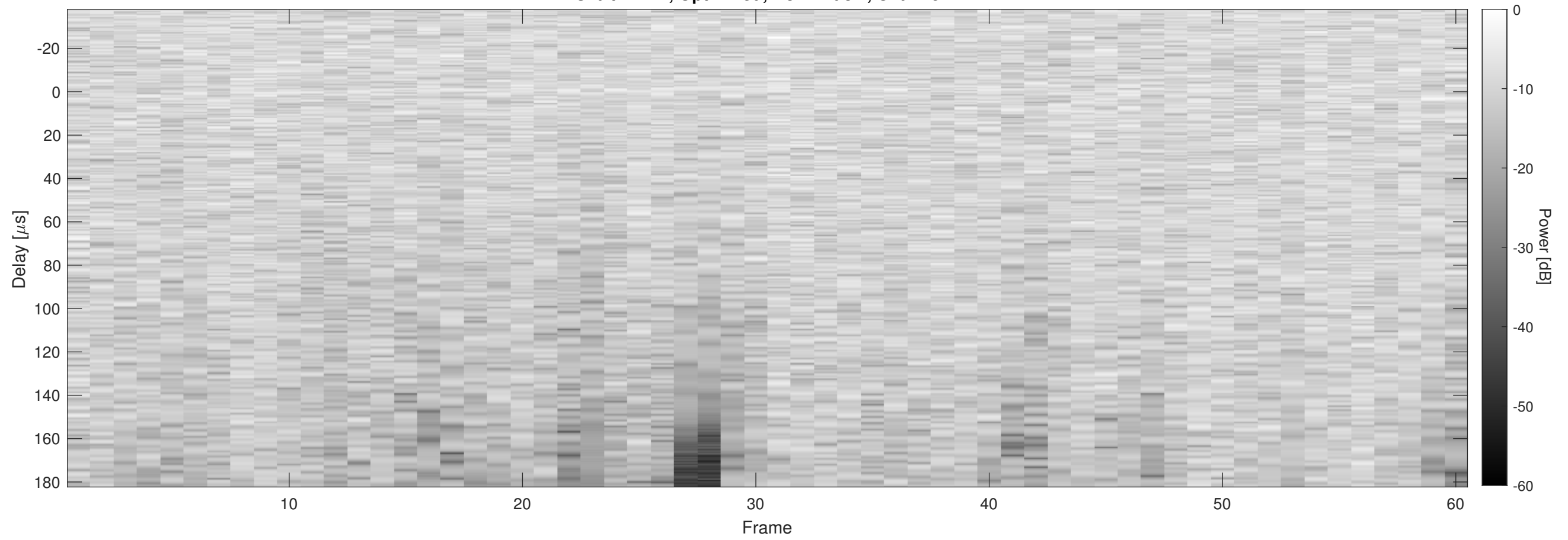
Orbit 22271, Optimized, No Window, Channel 2
