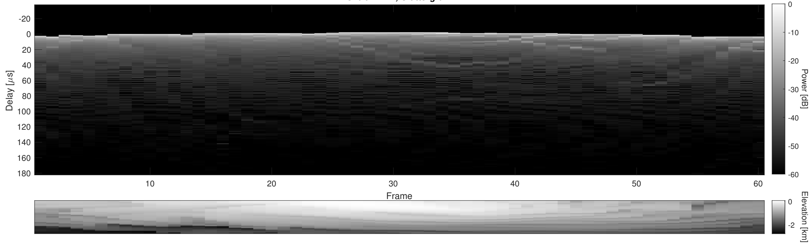
Orbit 22271, Cluttergram
