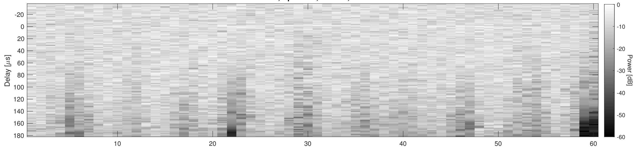
Orbit 22271, Cluttergram
