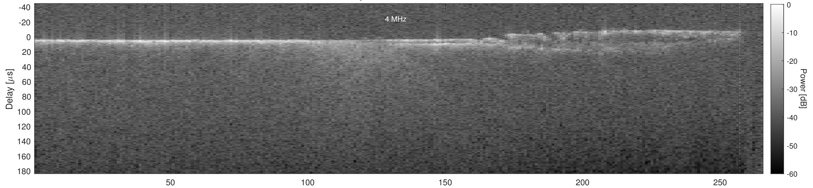
Orbit 22296, Cluttergram
