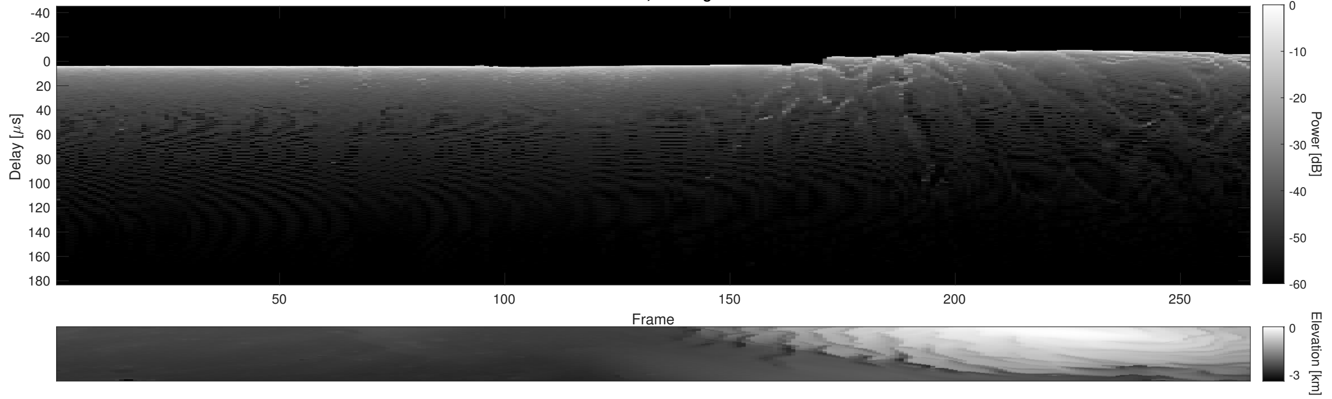
Orbit 22296, Cluttergram
