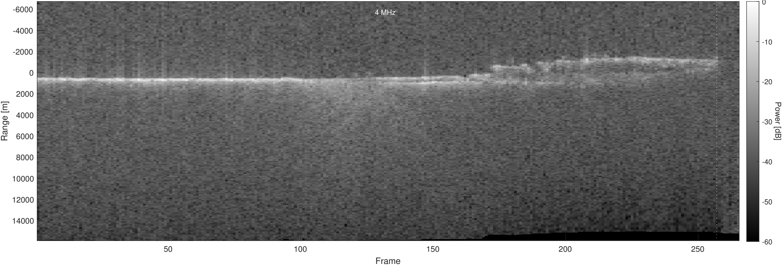
Orbit 22296, Optimized, No Window, Depth-Corrected, Channel 2
