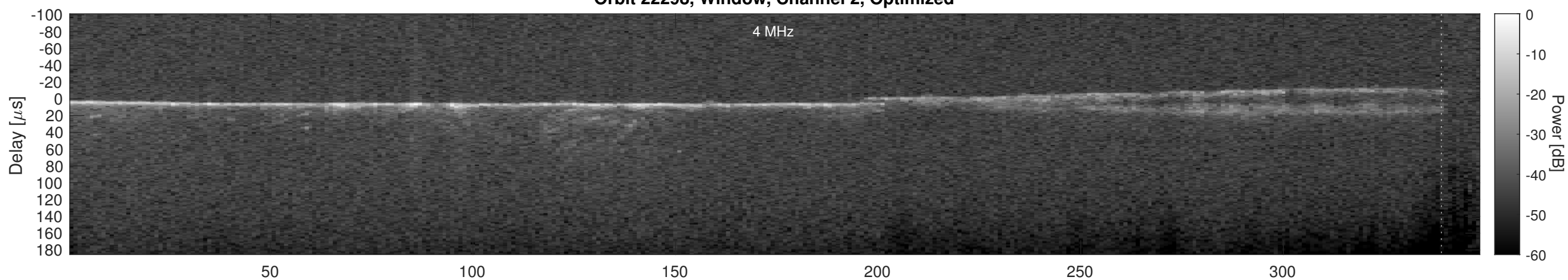
Orbit 22298, Cluttergram
