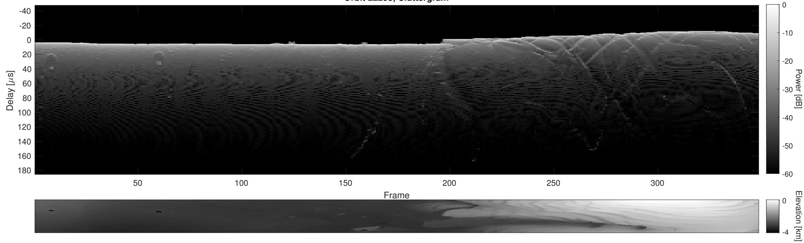
Orbit 22298, Cluttergram
