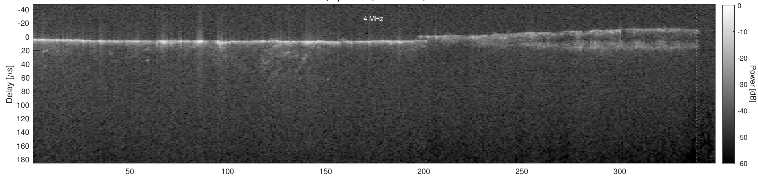
Orbit 22298, Cluttergram
