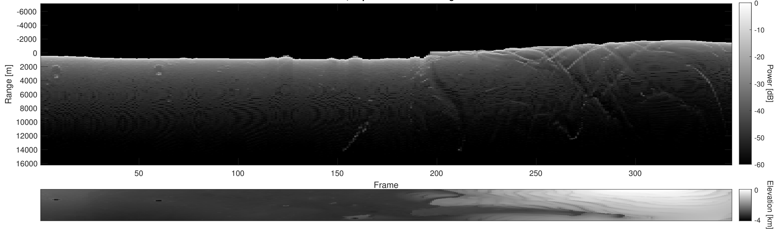
Orbit 22298, Depth-Corrected Cluttergram
