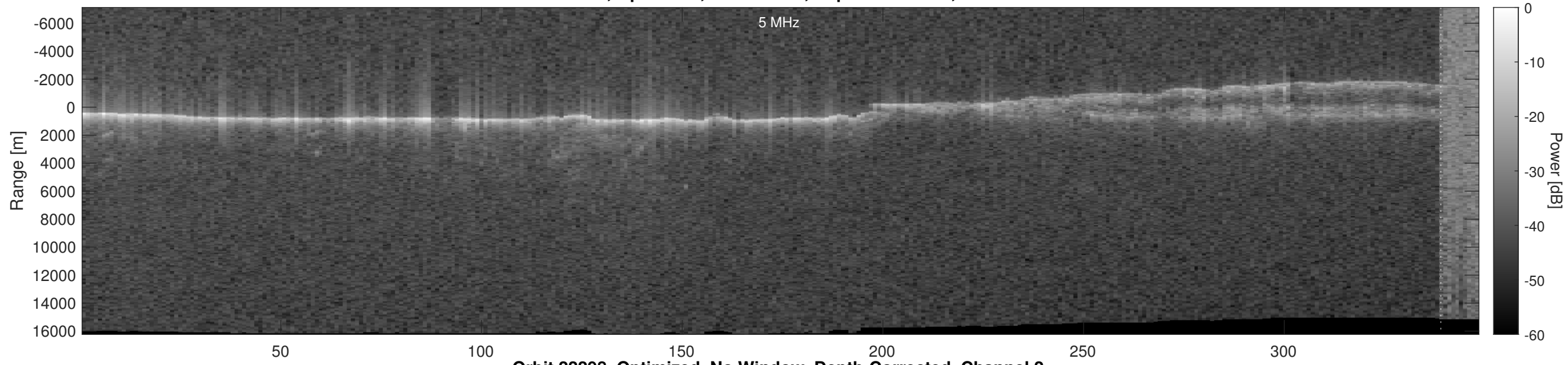
Orbit 22298, Optimized, No Window, Depth-Corrected, Channel 2
