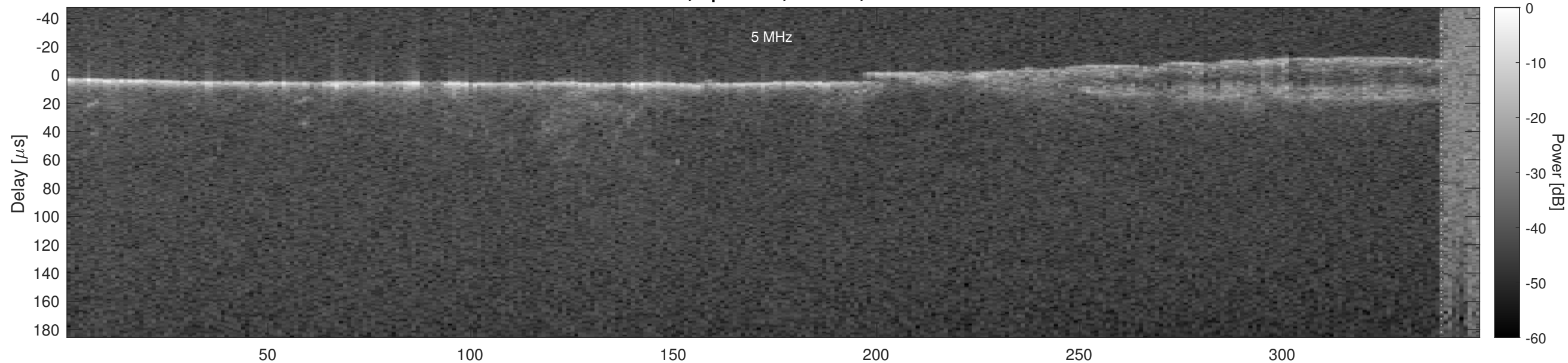
Orbit 22298, Optimized, Window, Channel 2
