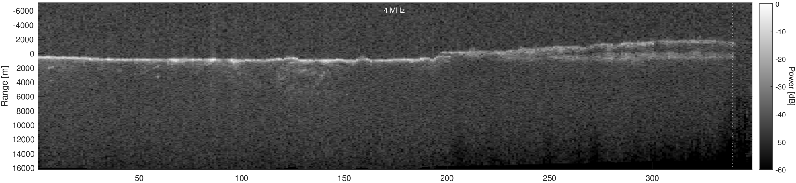
Orbit 22298, Depth-Corrected Cluttergram
