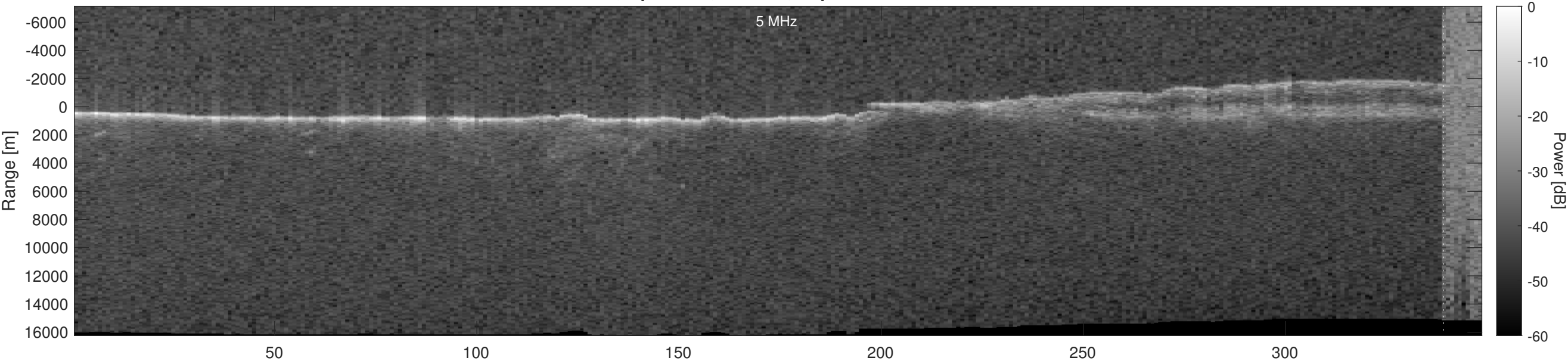
Orbit 22298, Optimized, Window, Depth-Corrected, Channel 2
