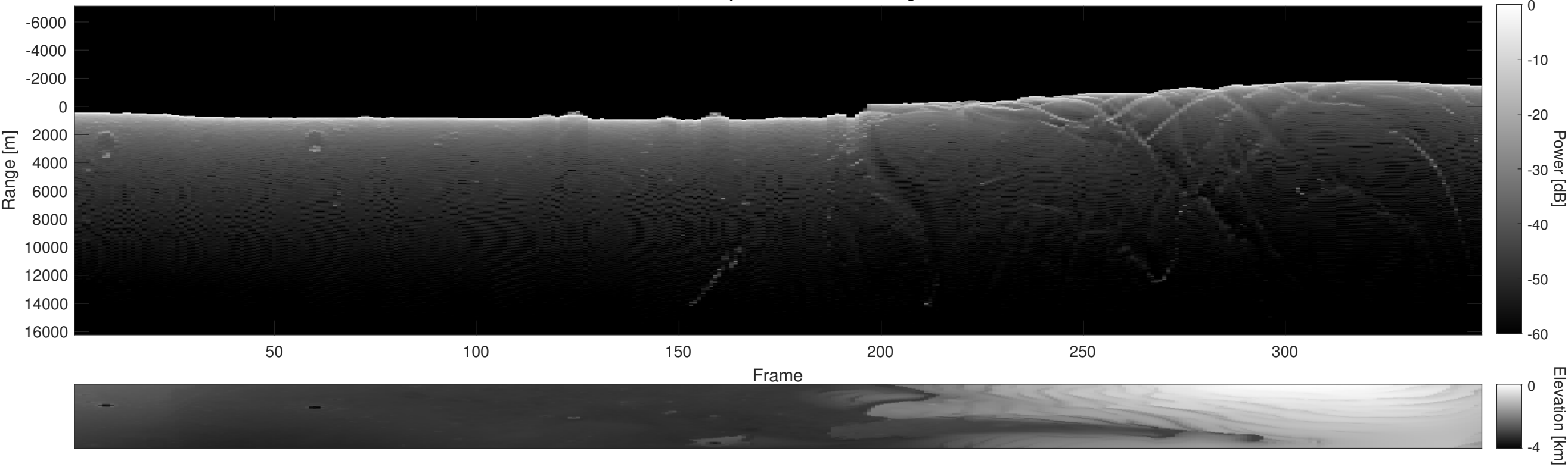
Orbit 22298, Depth-Corrected Cluttergram
