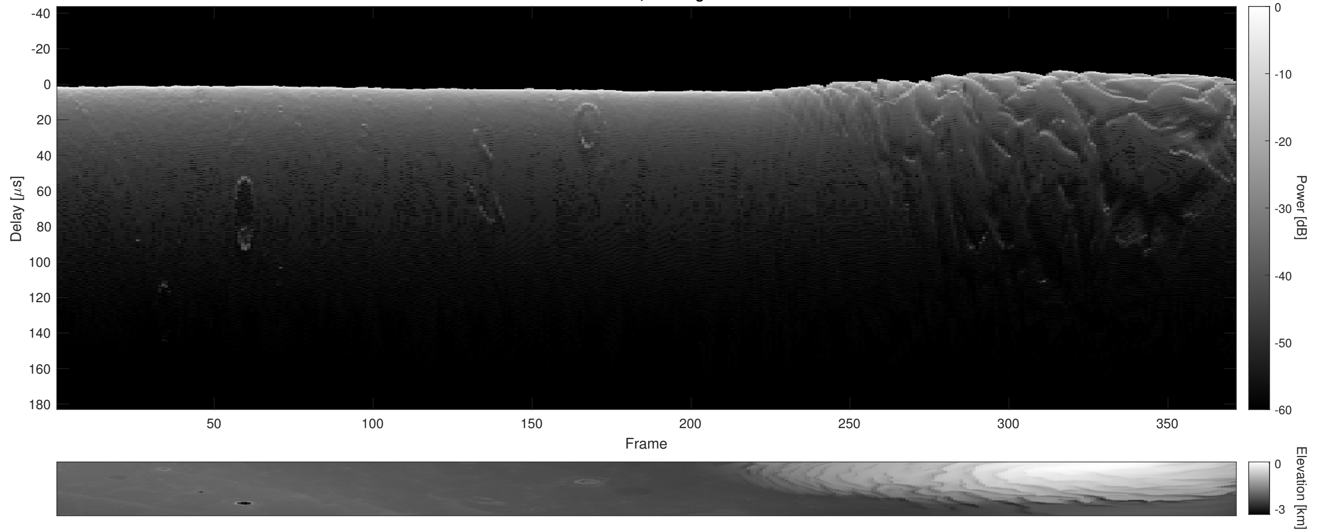
Orbit 22307, Cluttergram
