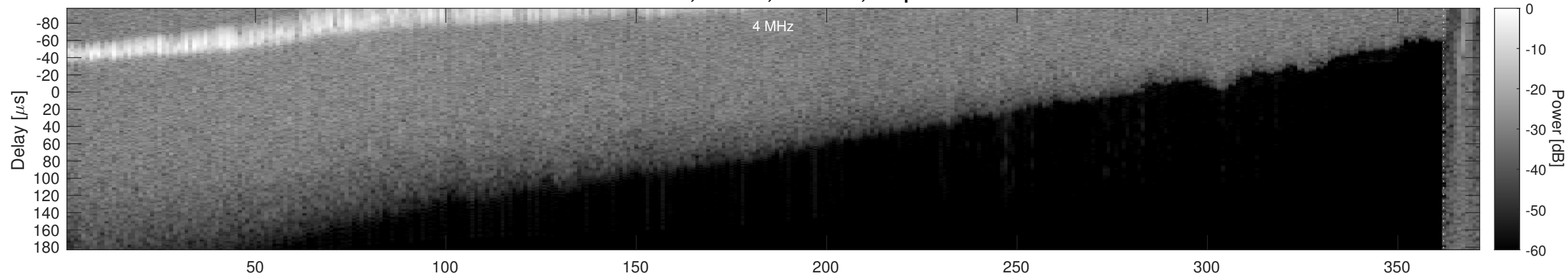
Orbit 22307, Window, Channel 2, Optimized
