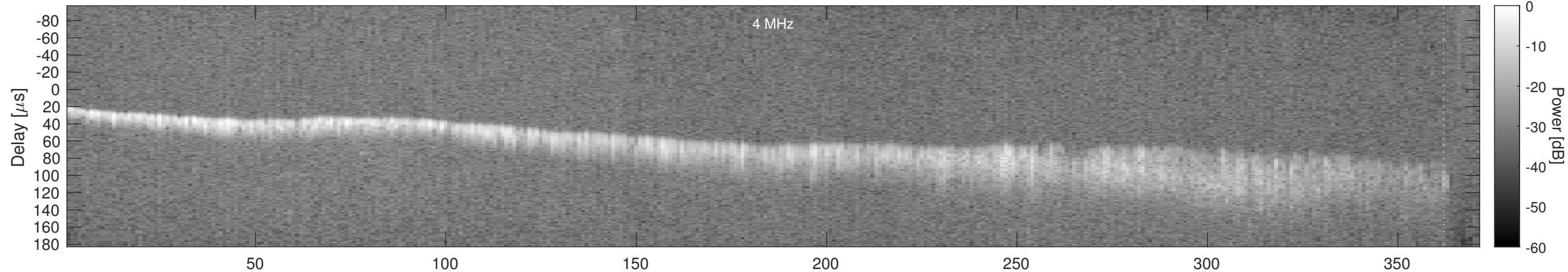
Orbit 22307, Window, Channel 2, Chapman
