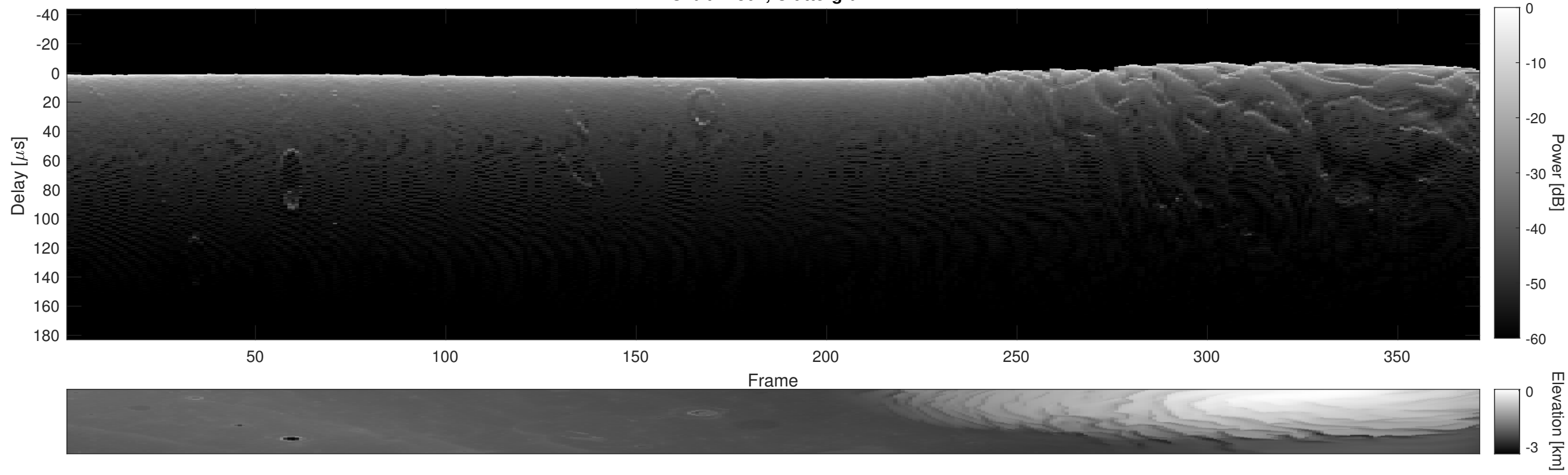
Orbit 22307, Cluttergram
