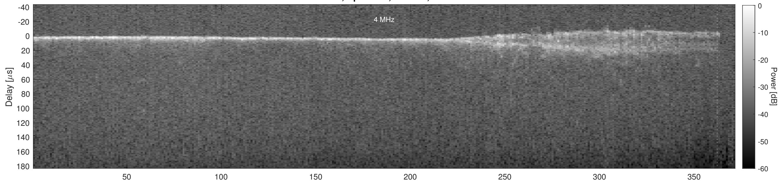
Orbit 22307, Cluttergram
