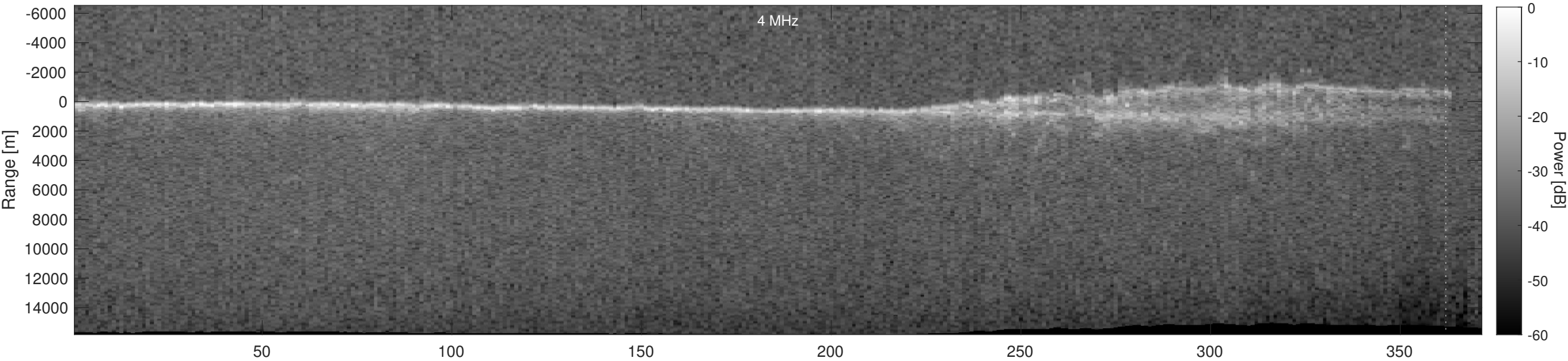
Orbit 22307, Depth-Corrected Cluttergram
