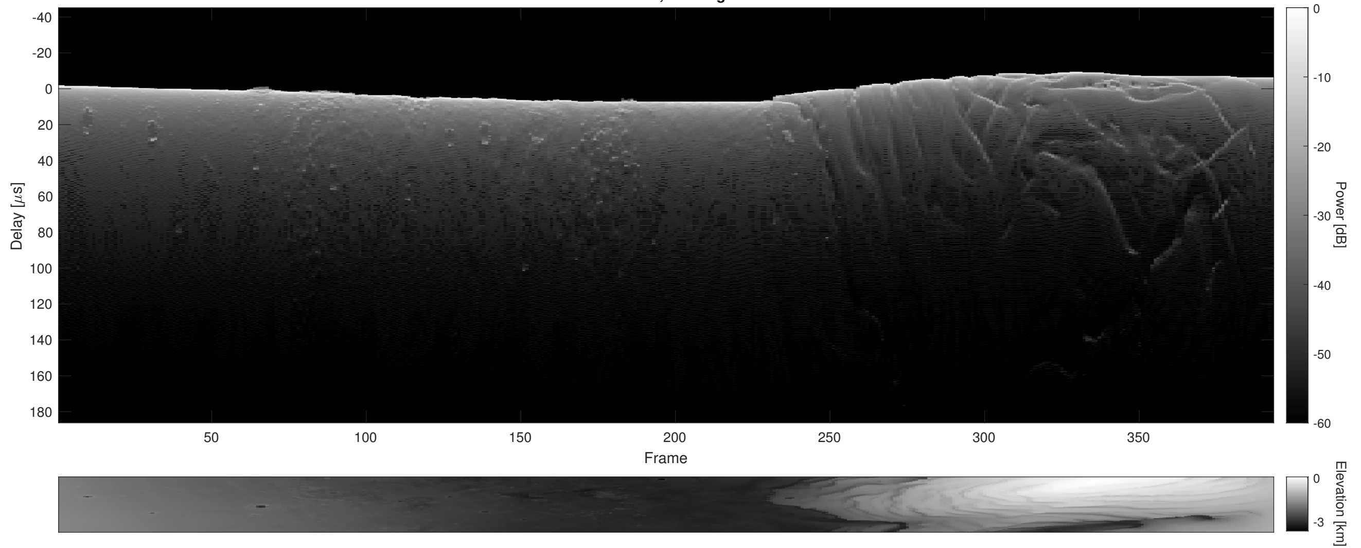
Orbit 22316, Cluttergram
