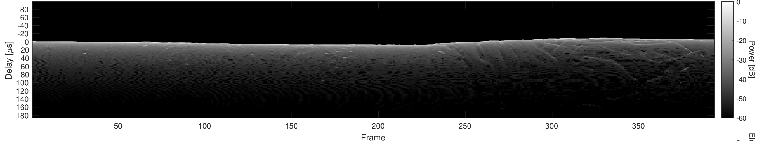
Orbit 22316, Cluttergram
