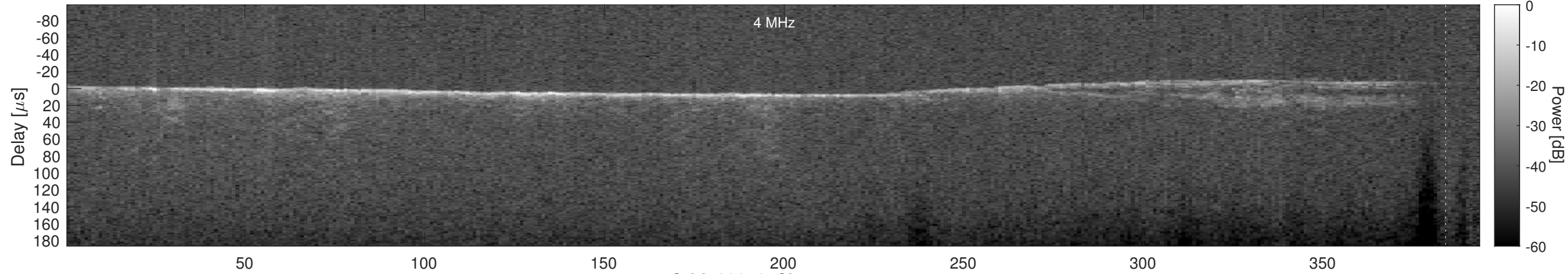
Orbit 22316, Cluttergram
