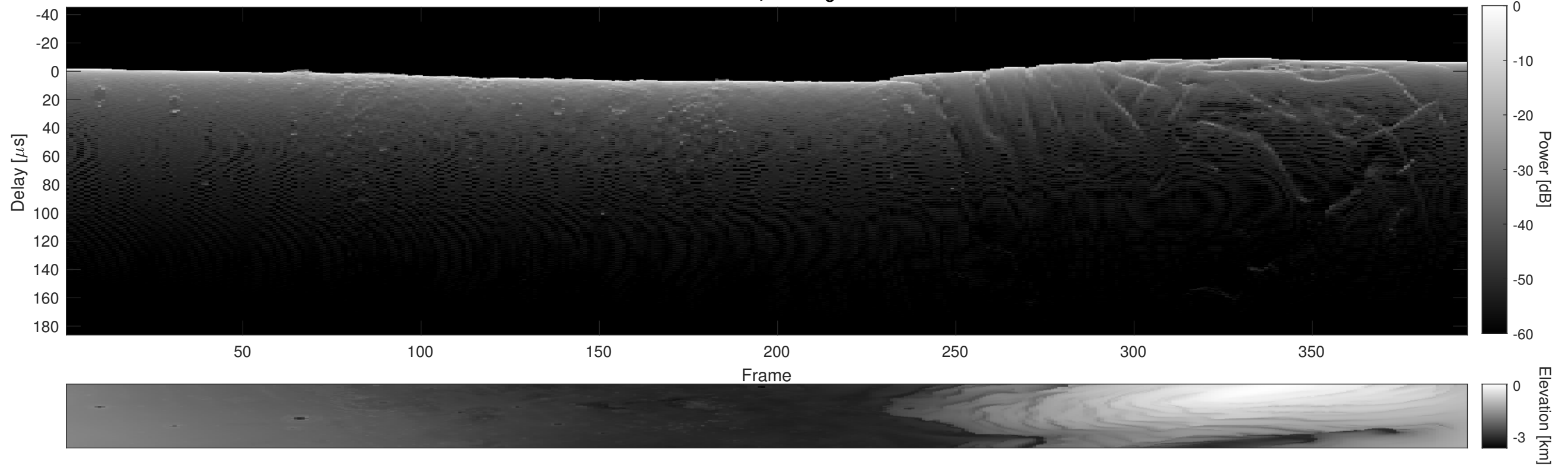
Orbit 22316, Cluttergram
