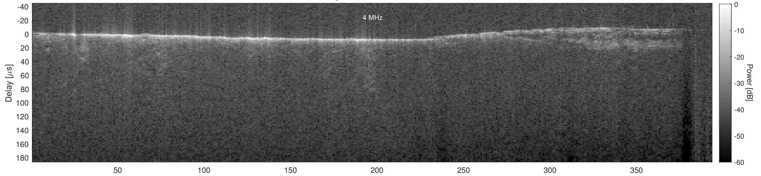
Orbit 22316, Cluttergram
