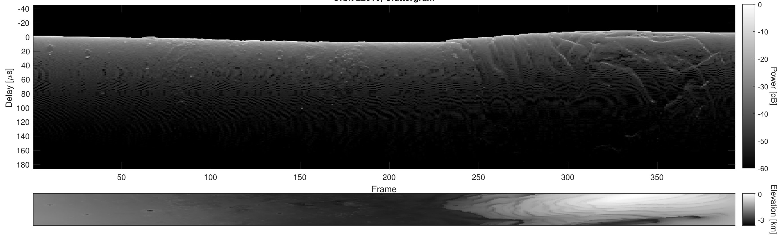
Orbit 22316, Cluttergram
