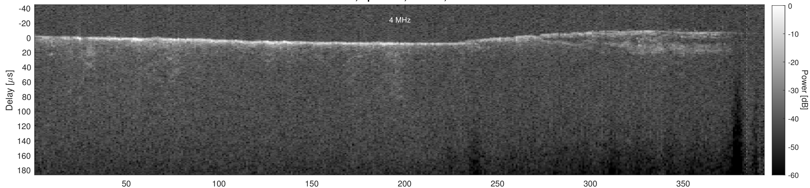
Orbit 22316, Cluttergram
