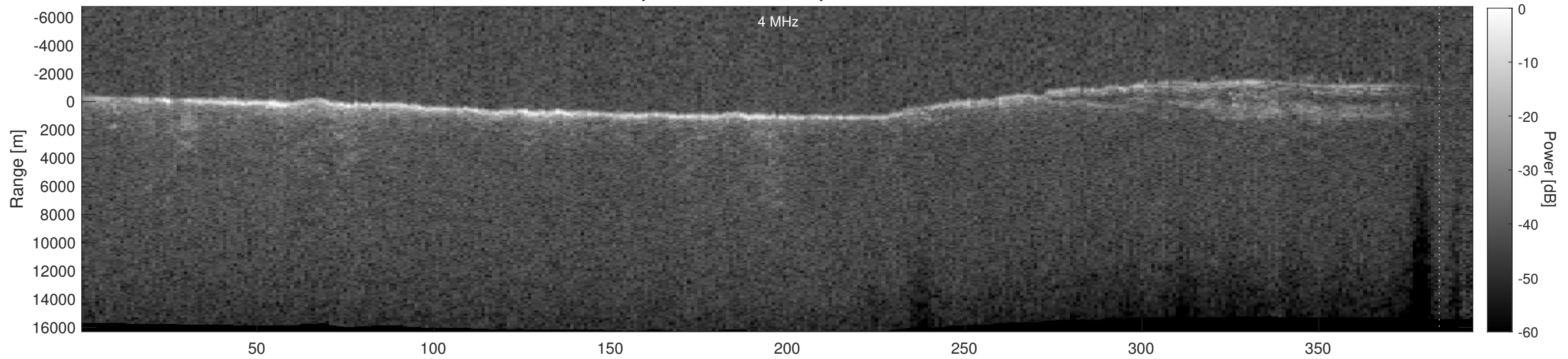
Orbit 22316, Depth-Corrected Cluttergram
