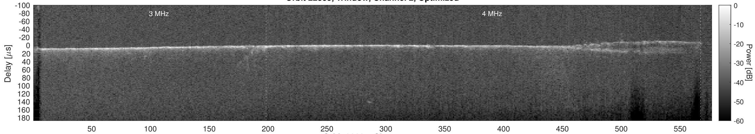
Orbit 22335, Cluttergram
