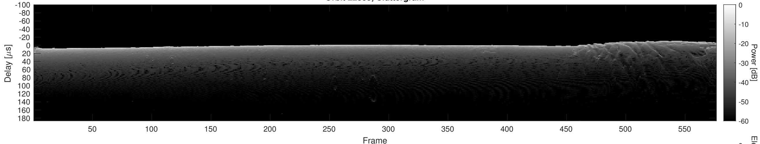
Orbit 22335, Cluttergram
