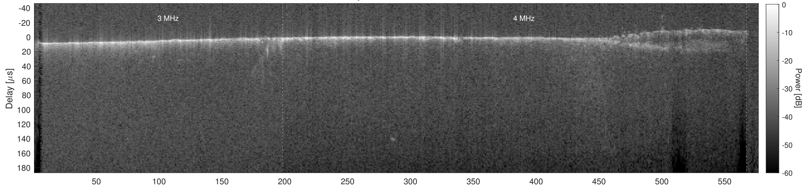
Orbit 22335, Cluttergram
