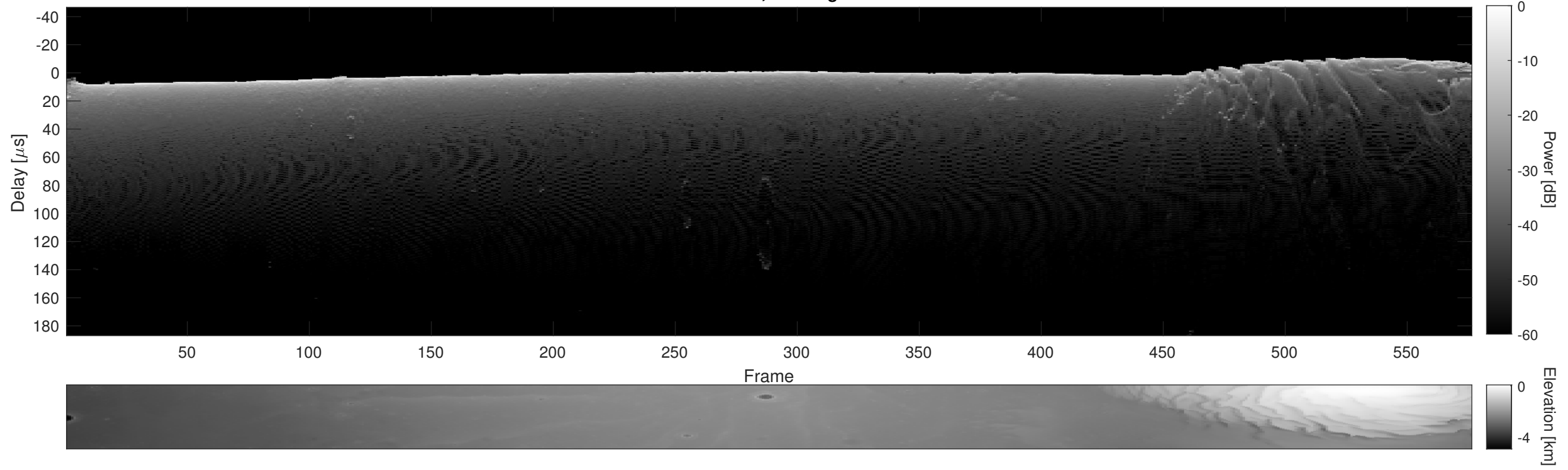
Orbit 22335, Cluttergram
