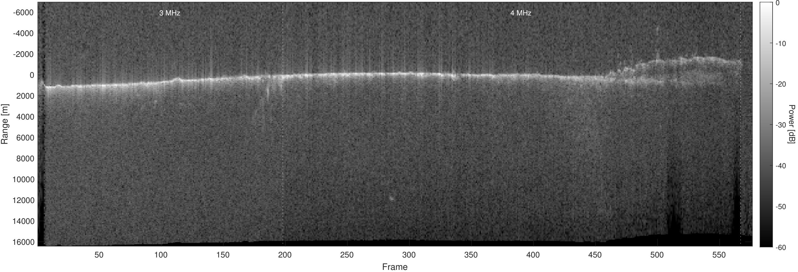
Orbit 22335, Optimized, No Window, Depth-Corrected, Channel 2
