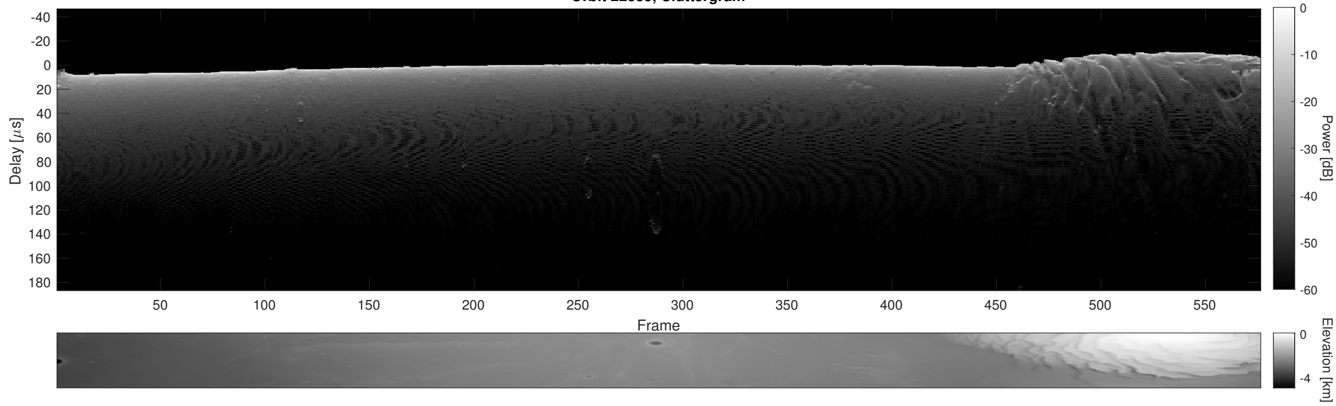
Orbit 22335, Cluttergram
