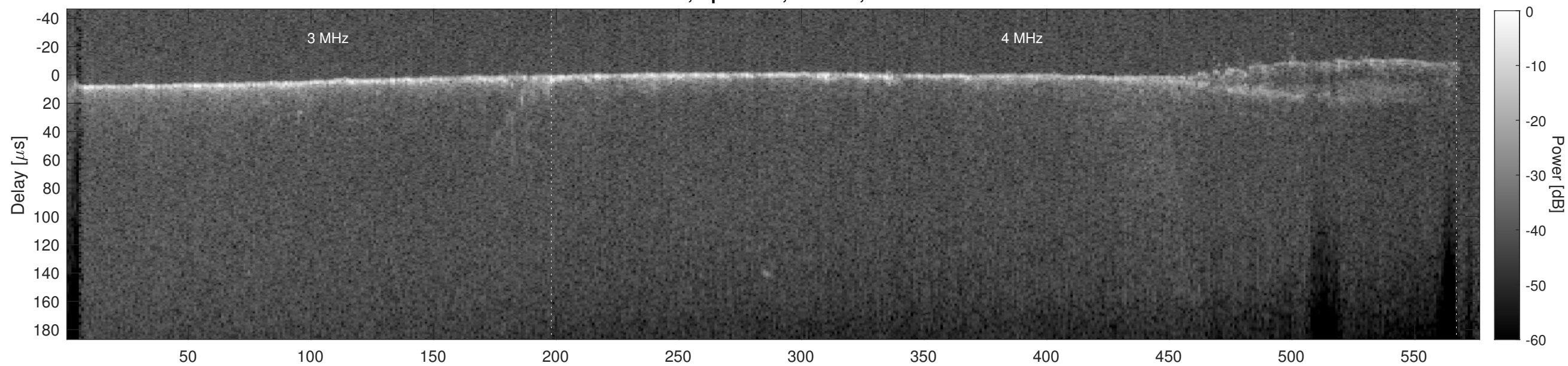
Orbit 22335, Cluttergram
