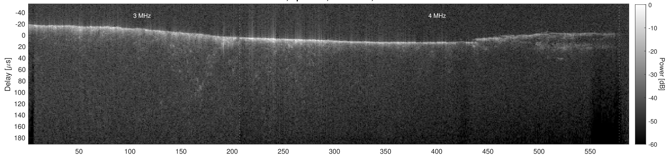
Orbit 22337, Cluttergram
