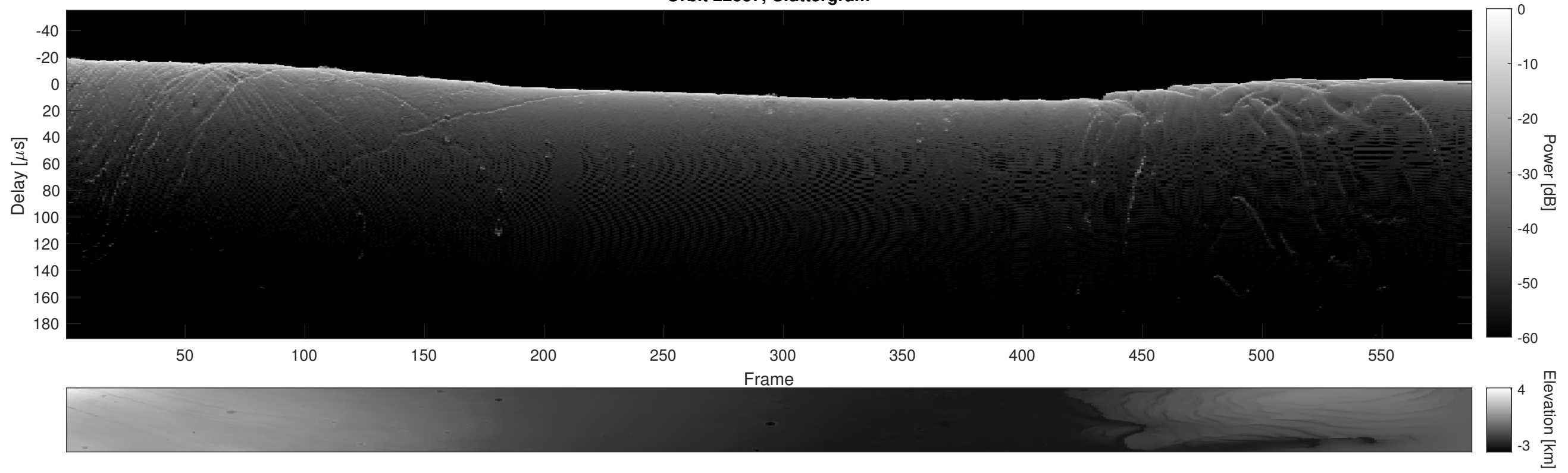
Orbit 22337, Cluttergram
