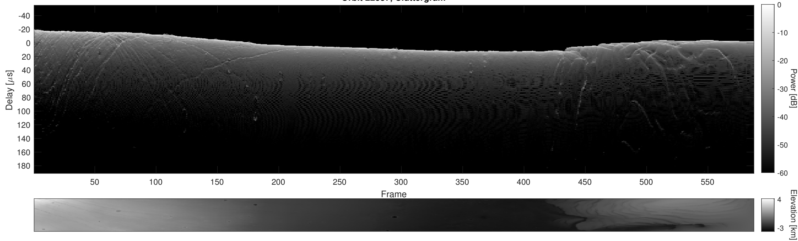
Orbit 22337, Cluttergram
