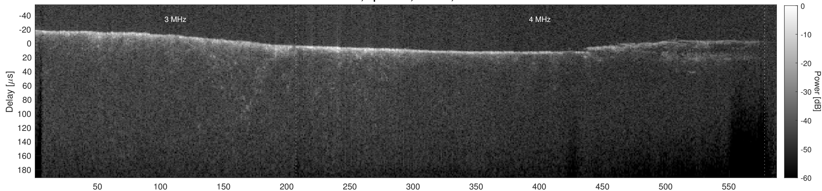
Orbit 22337, Cluttergram
