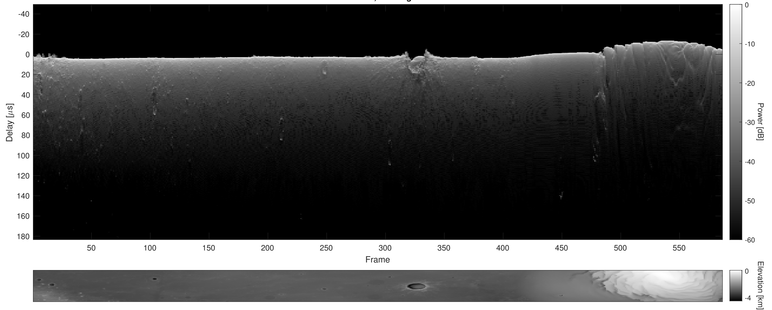
Orbit 22338, Cluttergram
